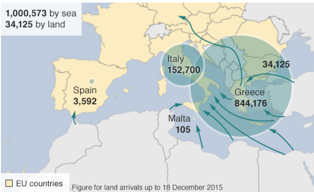
1 million arrivals by sea in 2015
